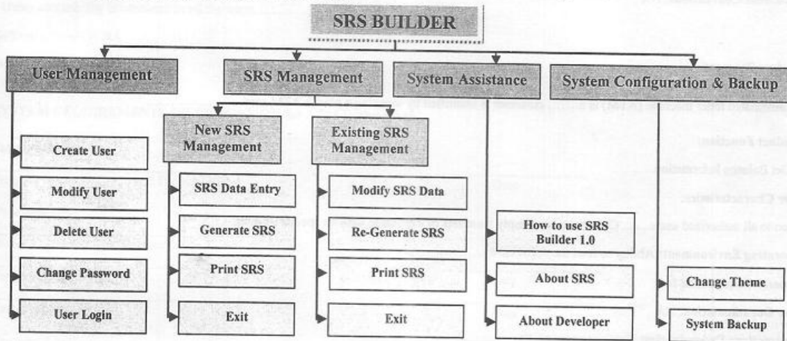
Figure 2: Function Hierarchy Diagram (FHD) of SRS Builder 1.0
